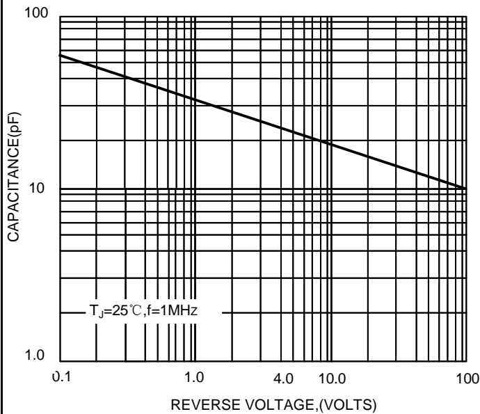
FIG.3-TYPICAL JUNCTION CAPACITANCE
